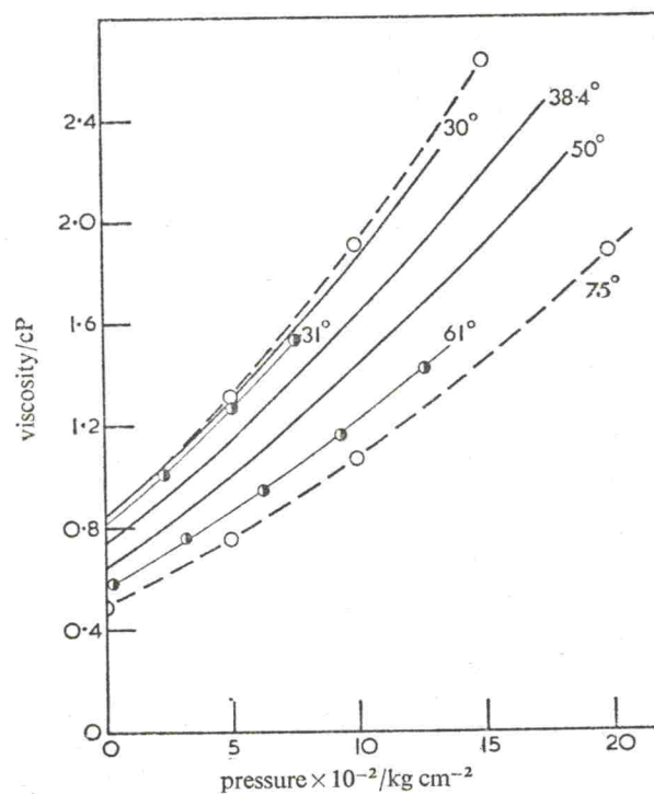
FIG. 8.—The viscosity of carbon tetrachloride. \bullet , Van Wijk et al. ; \circ , Bridgman 7 ; —, this work.
