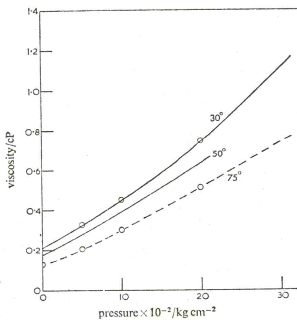
FIG. 9.—The viscosity of isopentane. \circ , Bridgman 7 ; —, this work.
